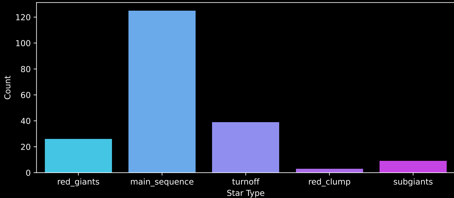
APOGEE DR17 Field: [119+63_MGA] Count plot of Star Type
