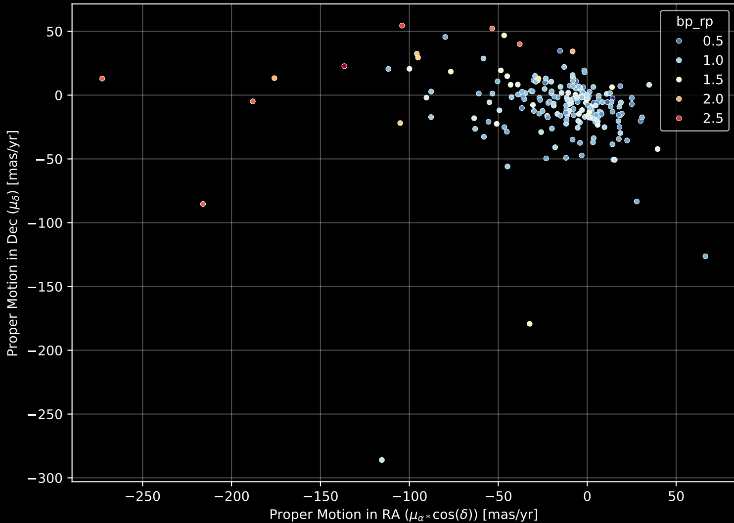
APOGEE DR17 Field: [119+63_MGA] Proper Motion Diagram (n= 202)
