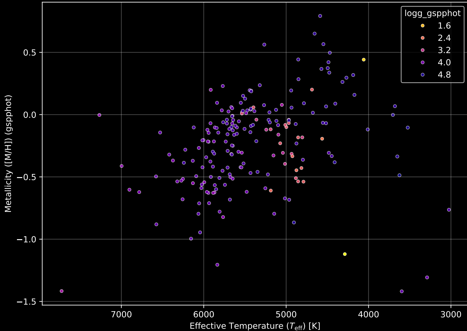
APOGEE DR17 Field: [119+63_MGA] Stellar Population Parameters (n= 202)
