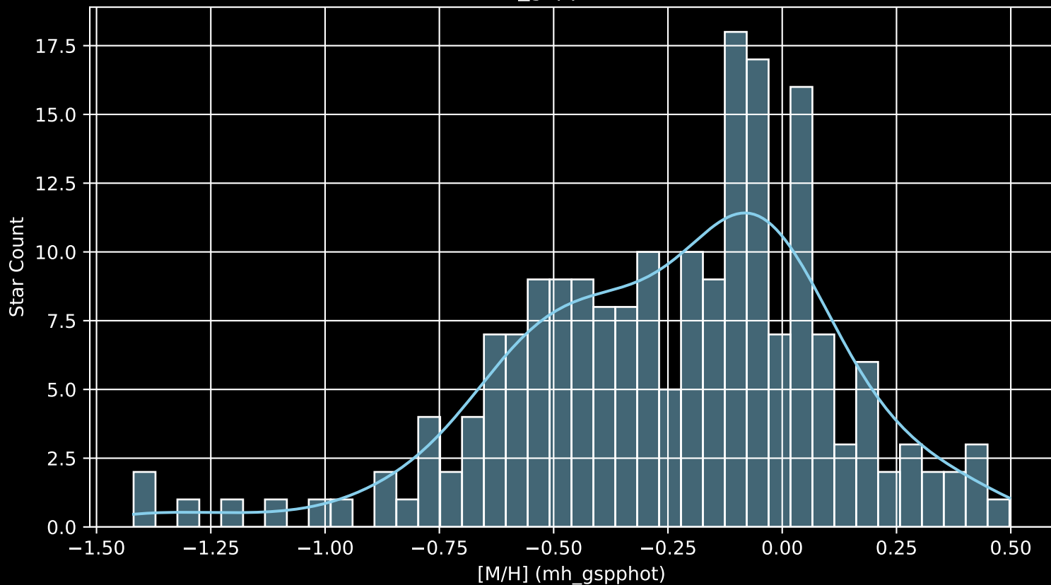
APOGEE DR17 Field: [119+63_MGA [M/H] (mh_gspphot) (n= 198)
