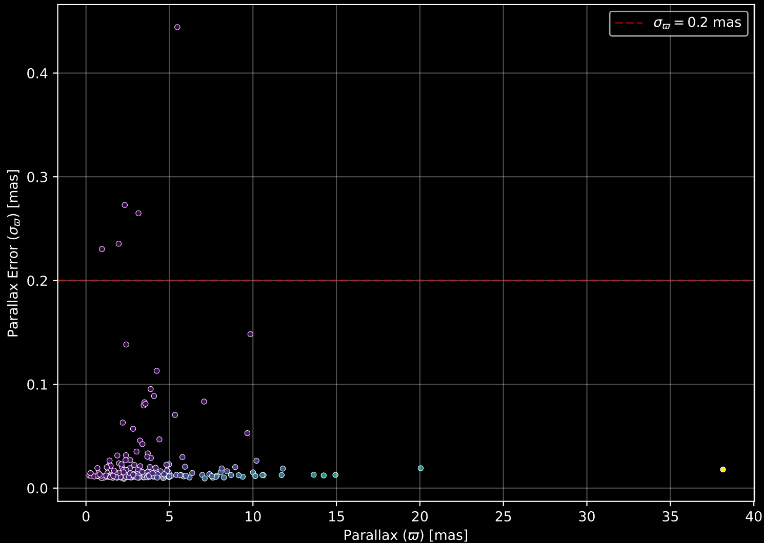
APOGEE DR17 Field: [119+63_MGA] Parallax Quality (n= 202)
