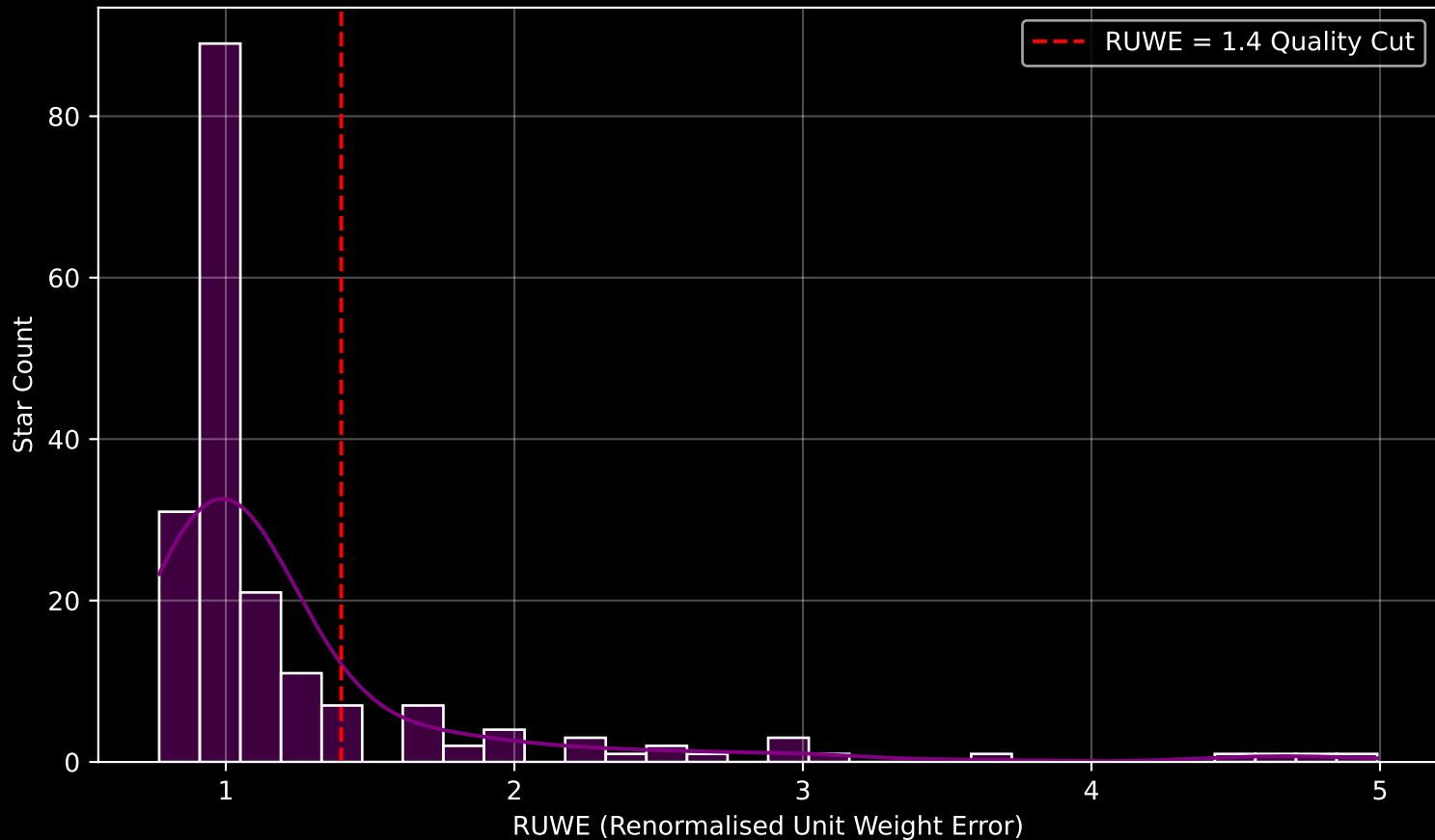
GAPOGEE DR17 Field [119+63_MGA] RUWE Distribution (n= 188)
